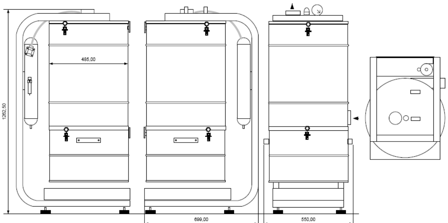
Dimensions (mm)
